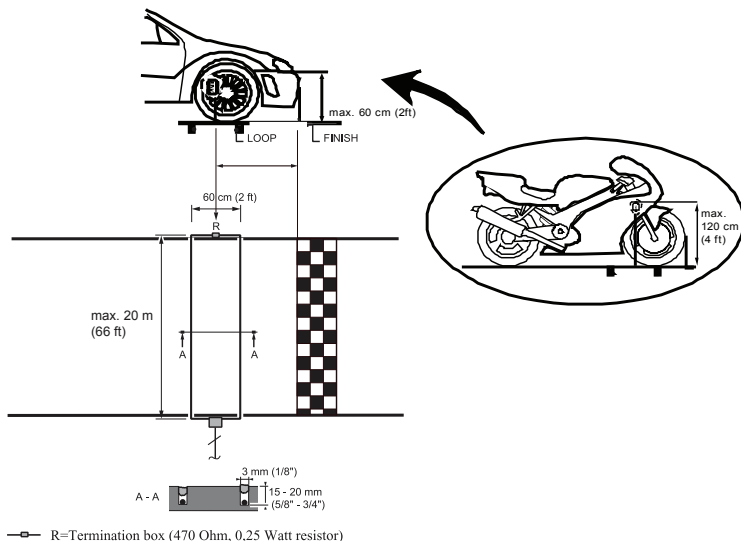
Figure 2.1 Detection loop installation overview
